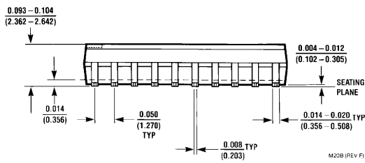
Molded Small Outline Package (M) Order Part LM2893M NS Package Number M20B
