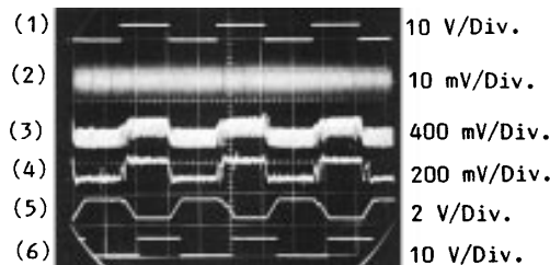
FIGURE 24. Oscilloscope revealing signals at several important nodes under weak signal ( 0.5 \text{ mV}_{\text{RMS}} ) conditions with SCR spikes on an otherwise quiet 115 V, 60 Hz power line. The signals are: 1) transmitted data, 2) RX carrier on the tuned transformer, 3) demodulated signal from the PLL after passing thru circuit of Figure 22 , 4) signal after RC lowpass, 5) data at impulse noise filter integrator, and 6) received data. Horizontal scale is 10 ms per div.
