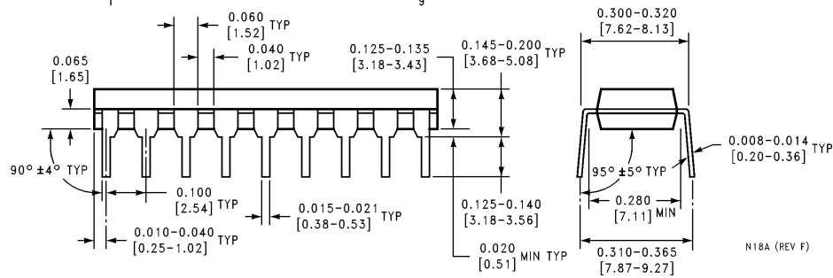
Molded Dual-In-Line Package (N) Order Part LM1893N NS Package Number N18A
