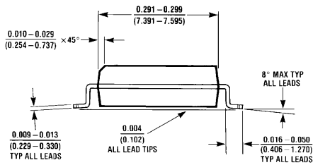
Molded Small Outline Package (M) Order Part LM2893M NS Package Number M20B
