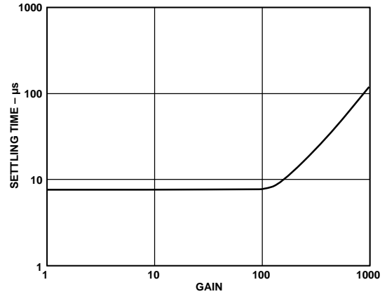
Figure 11. Settling Time to 0.1% vs. Gain, for a 10 V Step
