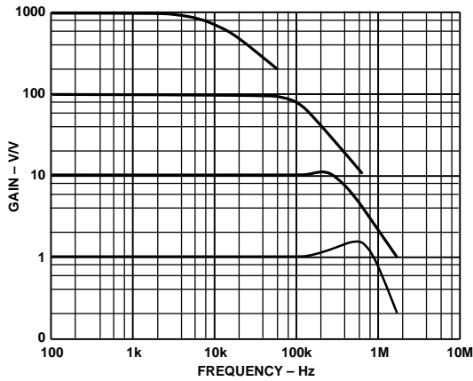
Figure 8. Gain vs. Frequency
