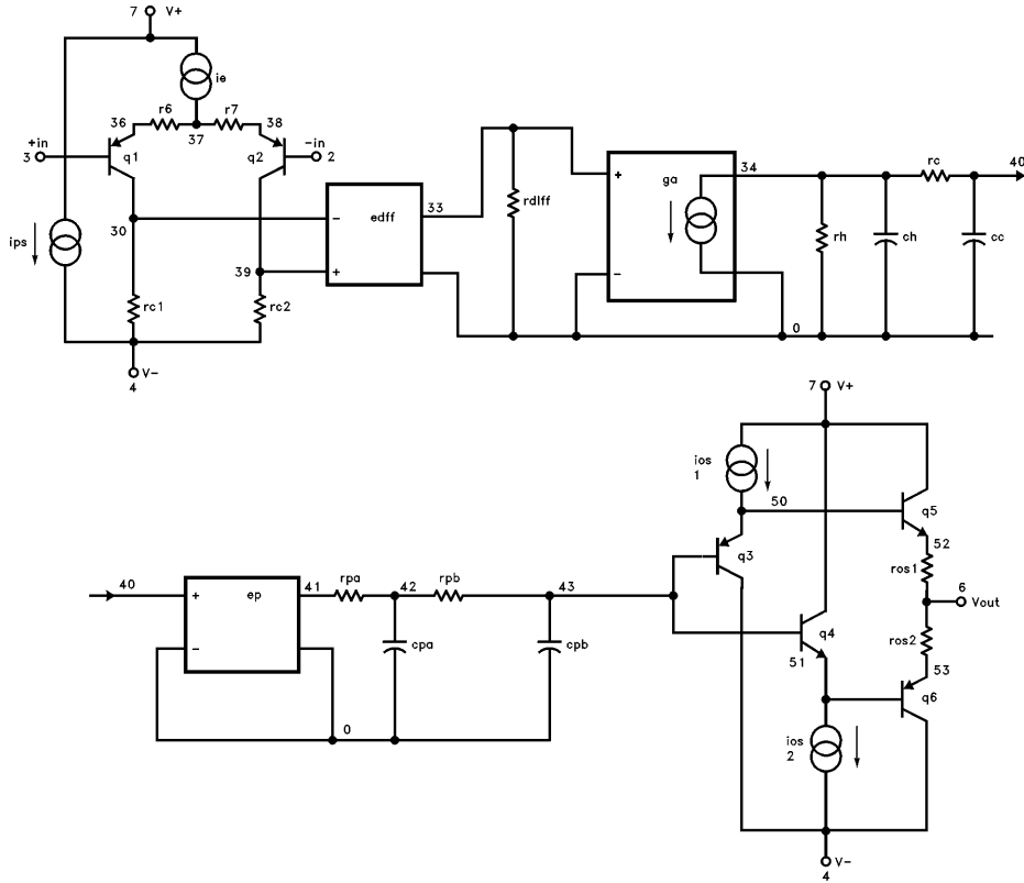
EL2244C/EL2444C Model
