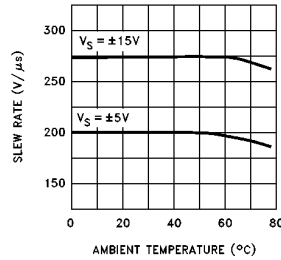
Slew Rate vs Temperature
