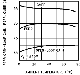
Open-Loop Gain, PSRR and CMRR vs Temperature
