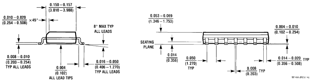
Order Number LF444CM See NS Package Number M14A
