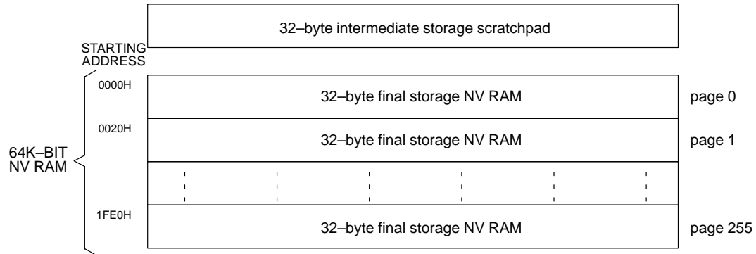
DS1996 MEMORY MAP Figure 5
