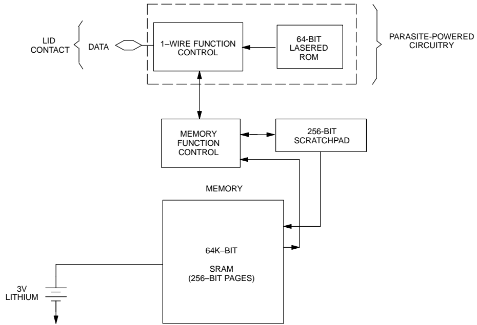
DS1996 BLOCK DIAGRAM Figure 1
