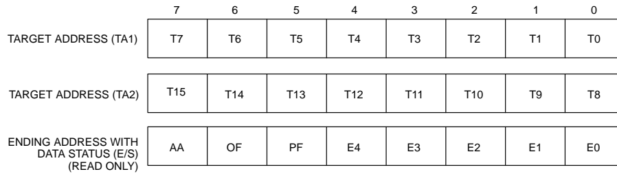
ADDRESS REGISTERS Figure 6
