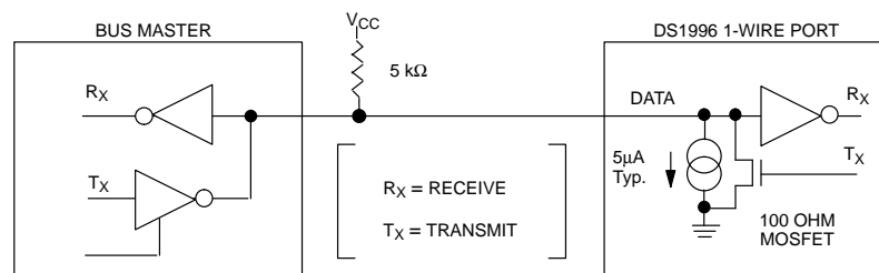
HARDWARE CONFIGURATION Figure 8
