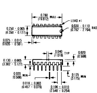
16 Lead Plastic DIP (PE) \theta_{JA} = 135^{\circ}\text{C/W} \theta_{JC} = 65^{\circ}\text{C/W}
