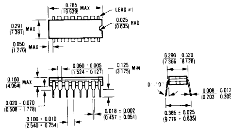
16 Lead Cerdip (JE) \theta_{JA} = 100^{\circ}\text{C/W} \theta_{JC} = 50^{\circ}\text{C/W}
