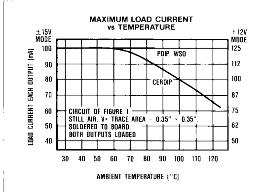
Figure 2. Maximum Load Current Vs. Temperature
