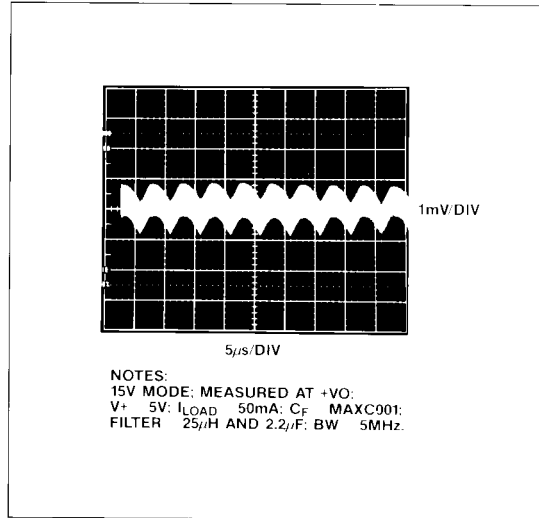
Figure 9. Output Noise Voltage with 1% Filter
