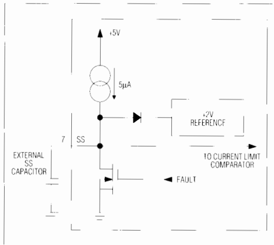
Figure 11. Soft-Start Equivalent Circuit
