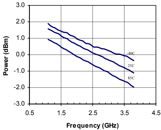
Figure 6. Output Power
