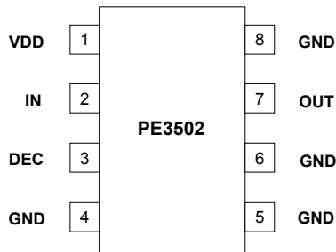
Figure 3. Pin Configuration
