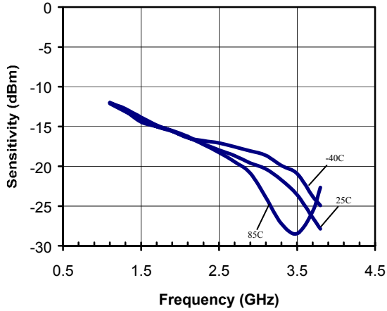
Figure 4. Input Sensitivity
