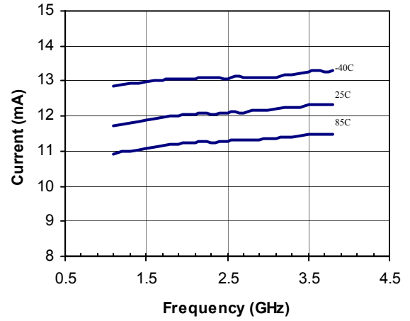
Figure 5. Device Current
