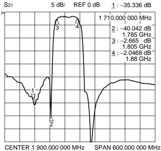
Filter 1 (Pass-band : 1805 MHz to 1880 MHz)
