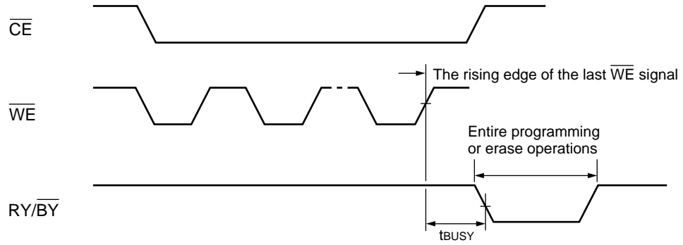
RY/\overline{BY} Timing Diagram during Program/Erase Operation Timing Diagram
