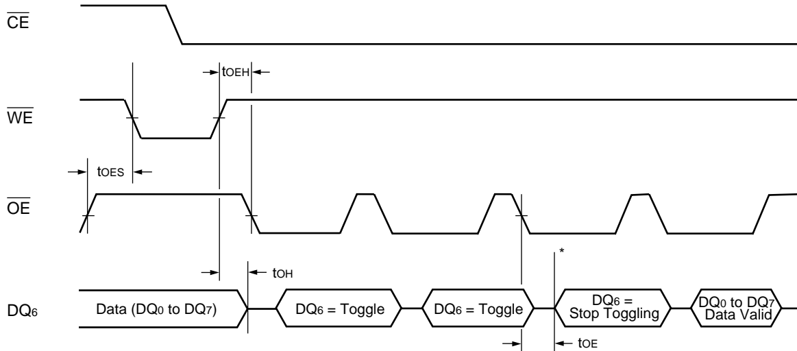
Figure 10 AC Waveforms for Toggle Bit I during Embedded Algorithm Operations
