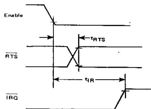
FIGURE 6 — REQUEST-TO-SEND DELAY AND INTERRUPT-REQUEST RELEASE TIMES
