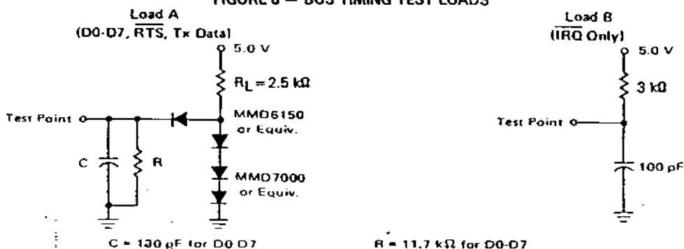
FIGURE 8 - BUS TIMING TEST LOADS
