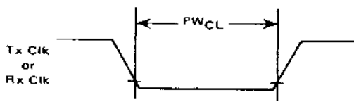
FIGURE 1 — CLOCK PULSE WIDTH, LOW-STATE
