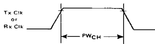
FIGURE 2 — CLOCK PULSE WIDTH, HIGH-STATE
